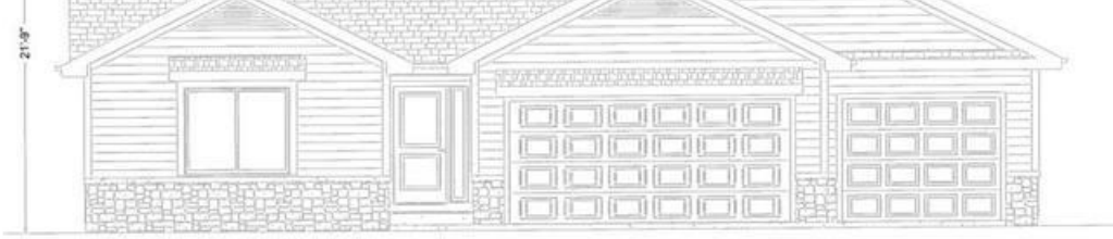
FRONT ELEVATION 1/4 = 1-0
